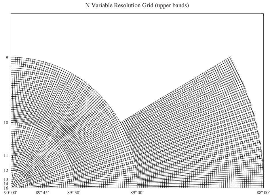
Fig. 3. NVRG tiling scheme. Cell structure of upper bands.
