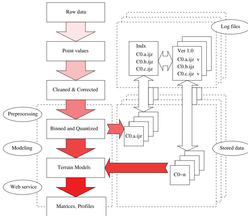
Fig. 4. Components and processes of the NVRG/Sarepta system.
